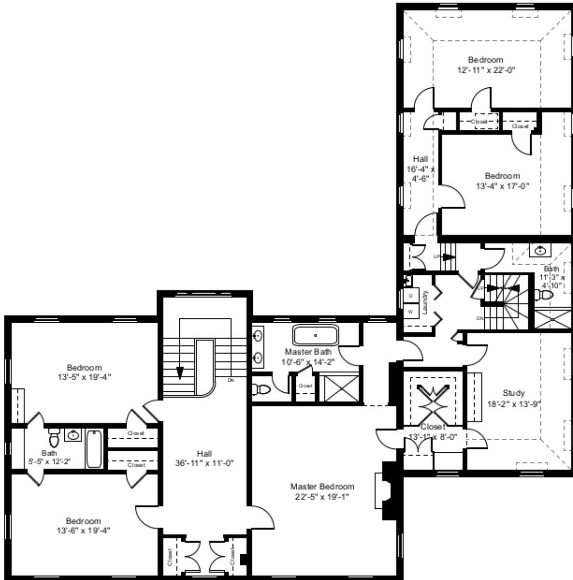
Second Floor Plan Ceiling Height = 9'-6"
